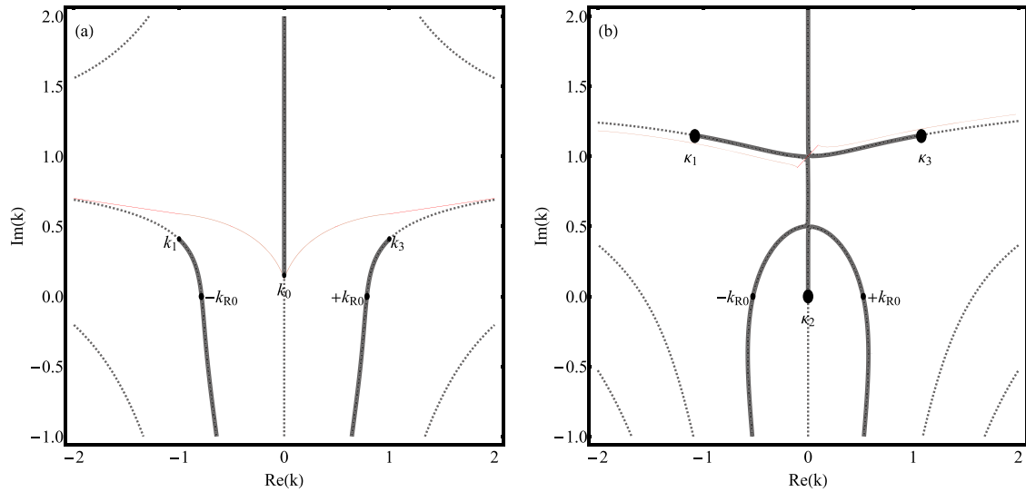
Figure 4. Contour plot of \arg ik e^{ikX-k^2} for \lambda = 10 and X = 2 (a) and X = 3 (b), in the complex k plane. Dotted and solid lines correspond to ik e^{ikX-k^2} \in \mathbb{R}_{\pm} respectively. The solid lines are branch cuts of \ln(1 + i\lambda k e^{ikX-k^2}) . A convenient choice for integration contours are the red lines while the points at which the branch cuts cross the real axis are denoted by \pm k_{R0} in accordance with equation (53). In panel (b) the branch points \kappa_i are denoted, while in panel (a) three branch points are arbitrarily denoted as k_i , i = 0, 1, 3 .
