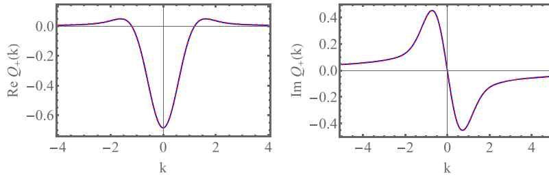
Figure 3. Analytical results for the real and imaginary parts of Q_+(k) , described by equations (37) and (39) (solid lines), versus numerical results (dashed lines), for \lambda = X = 1 , corresponding to J = 0.31 \dots
