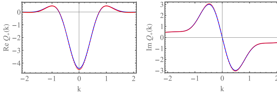
Figure 5. Analytical results for the real and imaginary parts of Q_+(k) for X > \sqrt{8} and \lambda > \lambda_{c2} , described by equations (49), (39) and (59) (solid lines), versus numerical results (markers). Parameters are \lambda = 20 and X = 3.5 , corresponding to J = 0.70 \dots
