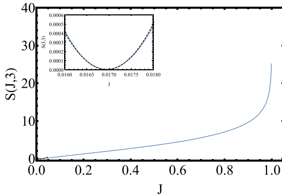
Figure 2. Action s(J, X = 3) as a function of J for X = 3 . Dashed line is the asymptote at J \rightarrow \bar{J} = \text{erfc}(3/2)/2 = 0.016\,947\dots , given by equation (69) below. The inset shows an enlargement of the asymptotic region.
