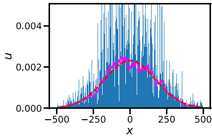
Figure 1. A Monte-Carlo simulation of the microscopic KMP model. Initially only one agent, at x = 0 , had a nonzero energy W = 1 . Plotted is the simulated energy profile u as a function of x at time t = 3 \times 10^4 (bars), its spatial average over each 50 consecutive lattice sites (solid line), and the theoretical mean-field profile (3) (dashed line).
