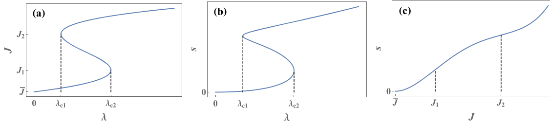
Figure 6. Schematic plots of (a) J(\lambda, X) , (b) s(\lambda, X) and (c) s(J, X) for X > \sqrt{8} and \lambda > 0 . Interestingly, J and s are not single-valued functions of \lambda , and s is not a convex function of J .
