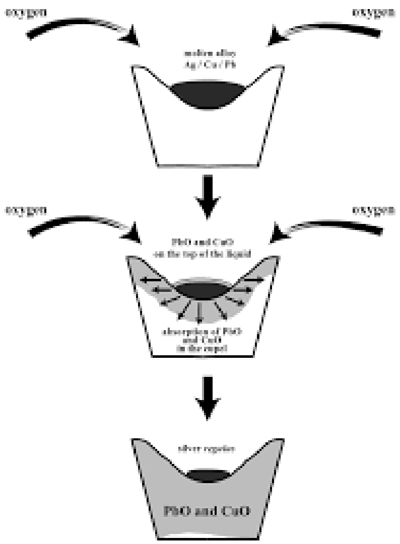
Cupellation- silver smelting process
