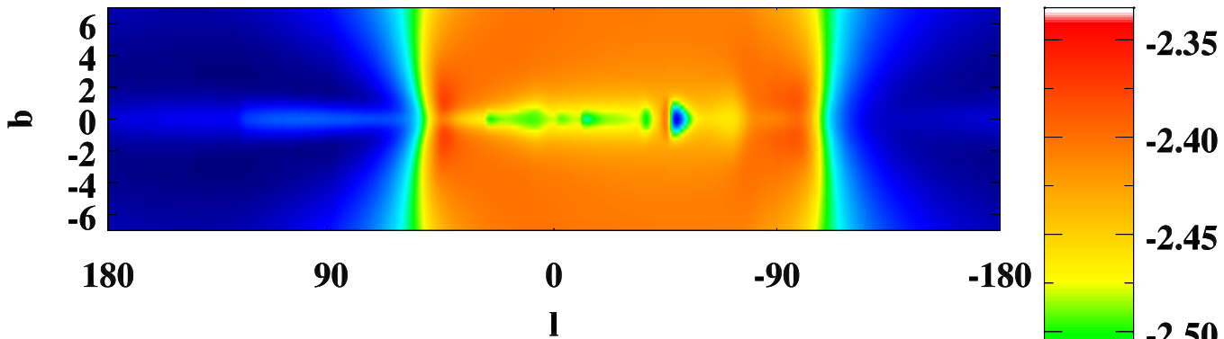
Spectral index 0.85-6.79 GeV: simulation
